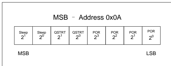
Fig7. MODE Register Format
