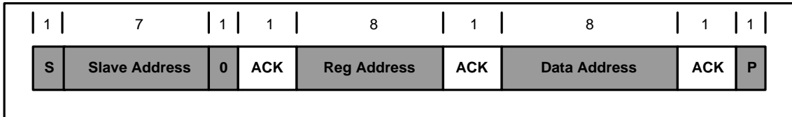
Figure 14: Single Write
